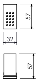
Cabide Hook, Percha Cod. 21.06.000.070.08
