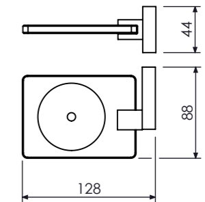
Saboneteira de Box Wall Mounted Glass Soap Holder, Jabonera para Ducha Cod. 21.30.077.126.08
