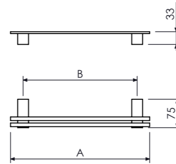
Toalheiro Towel Bar, Porta Toalla Barra 30cm 12" A=366 B=300 Cod. 21.35.002.096.08 60cm 24" A=666 B=600 21.35.005.096.08
