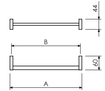
Toalheiro Towel Bar, Porta Toalla Barra 30cm 12" A=312 B=300 Cod. 21.35.002.126.08 60cm 24" A=612 B=600 Cod. 21.35.005.126.08
