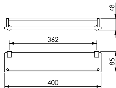
Porta Shampoo com Grade Glass Shelf with Rail, Porta Shampoo (vidrio con rejilla) Cod. 21.24.040.143.08
