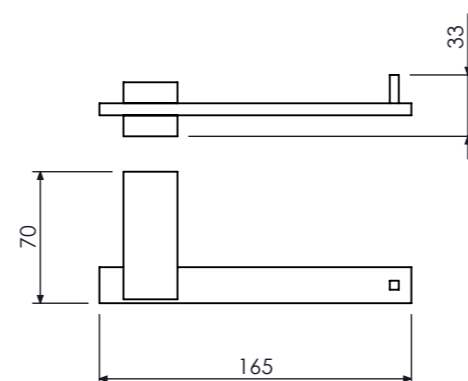
Papeleira Paper Holder, Porta Rollo Cod. 21.19.000.057.08
