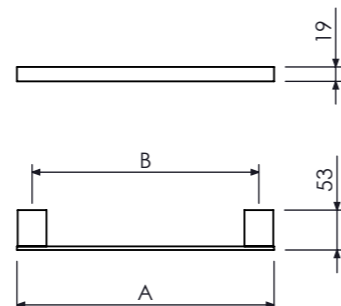
Toalheiro Towel Bar, Porta Toalla Barra 30cm 12" A=340 B=300 Cod. 21.35.002.129.08 60cm 24" A=640 B=600 Cod. 21.35.005.129.08
