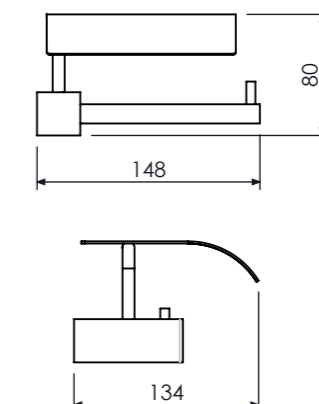
Papeleira com Capa Paper Holder with Cover, Porta Rollo con Capa Cod. 21.19.038.120.08
