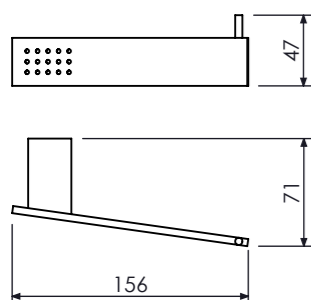
Papeleira Paper Holder, Porta Rollo Cod. 21.19.000.070.08
