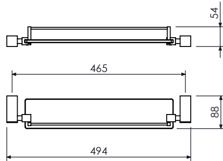
Porta Shampoo com Grade Glass Shelf with Rail, Porta Shampoo (vidrio con rejilla) Cod. 21.24.040.120.08
