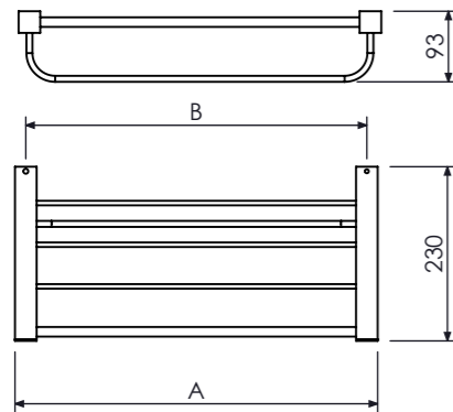
Toalheiro Rack com Alça Towel Rack with Towel Bar, Rack para Toallas con Barra 45cm 18" A=479 B=450 Cod. 21.35.085.120.08 60cm 24" A=629 B=600 Cod. 21.35.086.120.08
