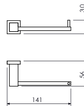
Papeleira Paper Holder, Porta Rollo Cod. 21.19.000.061.08
