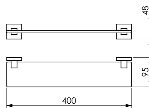
Porta Shampoo Glass Shelf, Porta Shampoo Cod. 21.24.000.144.08
