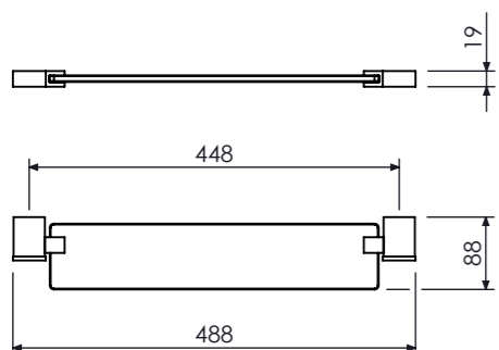
Porta Shampoo Glass Shelf, Porta Shampoo Cod. 21.24.000.129.08
