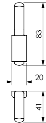
Cabide Hook, Percha Cod. 21.06.000.143.08
