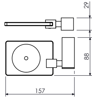
Saboneteira de Box Wall Mounted Glass Soap Holder, Jabonera para Ducha Cod. 21.30.077.120.08
