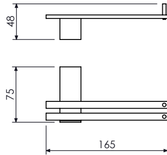
Papeleira Paper Holder, Porta Rollo Cod. 21.19.000.096.08
