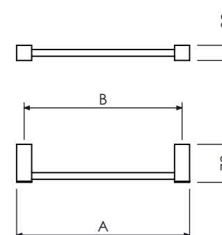
Toalheiro Towel Bar, Porta Toalla Barra 20cm 8" A=229 B=200 Cod. 21.35.001.120.08 30cm 12" A=329 B=300 Cod. 21.35.002.120.08 45cm 18" A=479 B=450 Cod. 21.35.003.120.08 60cm 24" A=629 B=600 Cod. 21.35.005.120.08
