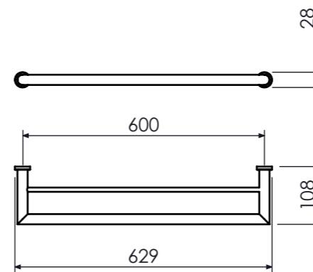
Toalheiro Duplo Double Towel Bar, Porta Toalla Barra Doble 60cm Cod. 21.35.069.063.08
