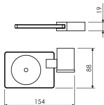
Saboneteira de Box Wall Mounted Glass Soap Holder, Jabonera para Ducha Cod. 21.30.077.129.08
