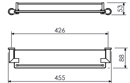
Porta Shampoo com Grade Glass Shelf with Rail, Porta Shampoo (vidrio con rejilla) Cod. 21.19.000.063.08
