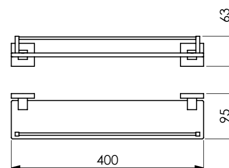
Porta Shampoo com Grade Glass Shelf with Rail, Porta Shampoo (vidrio con rejilla) Cod. 21.24.040.144.08
