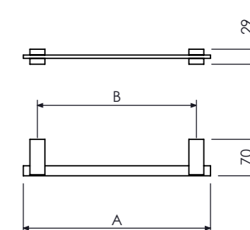
Toalheiro Towel Bar, Porta Toalla Barra 30cm 12" A= 357 B=303 Cod. 21.35.002.057.08 60cm 24" A= 657 B=603 Cod. 21.35.005.057.08
