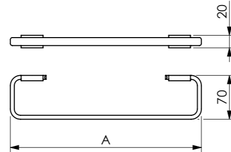
Toalheiro Towel Bar, Porta Toalla Barra 30cm 12" A=342 B=300 C=81 Cod. 21.35.002.143.08 60cm 24" A=642 B=600 C=88 Cod. 21.35.005.143.08
