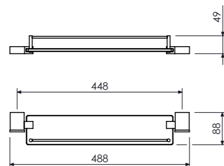
Porta Shampoo com Grade Glass Shelf with Rail, Porta Shampoo Cod. 21.24.040.129.08
