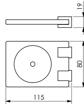
Saboneteira de Box Wall Mounted Glass Soap Holder, Jabonera para Ducha Cod. 21.30.077.143.08
