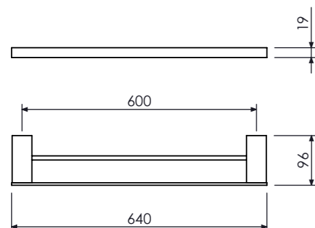
Toalheiro Duplo Double Towel Bar, Porta Toalla Barra Doble 60cm Cod. 21.35.069.129.08
