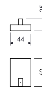
Cabide Hook, Percha Cod. 21.06.000.126.08
