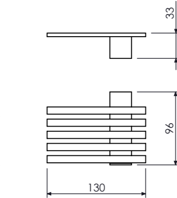
Saboneteira Soap Rack, Jabonera Cod. 21.30.077.096.08
