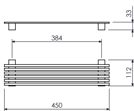
Porta Shampoo Shampoo Rack, Porta Shampoo Cod. 21.24.000.096.08
