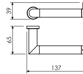
Papeleira Paper Holder, Porta Rollo Cod. 21.19.000.063.08
