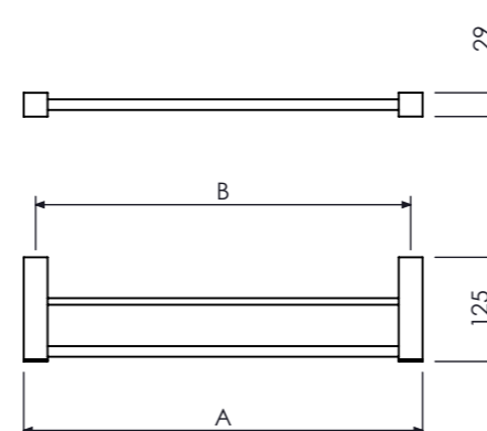
Toalheiro Duplo Double Towel Bar, Porta Toalla Barra Doble 45cm 18" A=479 B=450 Cod. 21.35.068.120.08 60cm 24" A=629 B=600 Cod. 21.35.069.120.08
