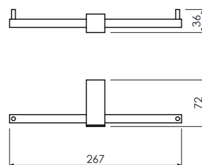
Papeleira Dupla Double Paper Holder, Porta Rollo Doble Cod. 21.19.067.120.08
