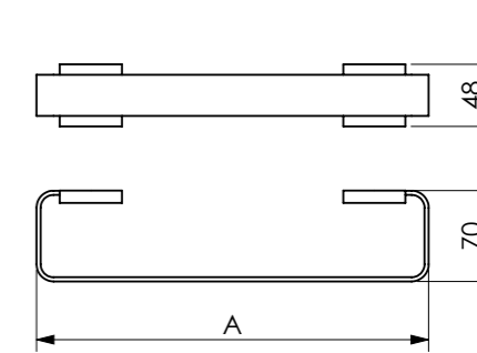
Toalheiro Towel Bar, Porta Toalla Barra 30cm 18" A=420 B=300 Cod. 21.35.002.144.08 60cm 24" A=720 B=600 Cod. 21.35.005.144.08
