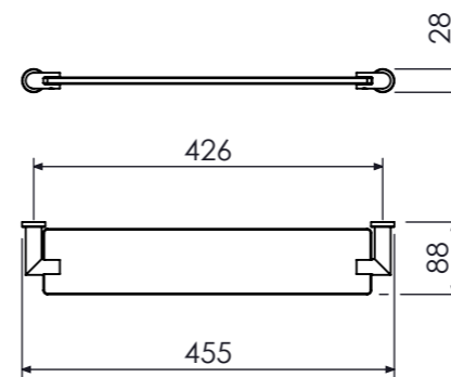
Porta Shampoo Glass Shelf, Porta Shampoo Cod. 21.24.000.063.08
